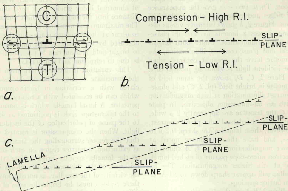
FIG. 3.— a , diagrammatic representation of edge dislocation in a simple lattice, showing main components of its stress field. The lattice is in compression (C) on the side of the slip plane with the extra half-plane and in tension (T) on the other; there are shear stresses on the slip plane with the senses shown. b , array of parallel edge dislocations locked in the slip plane, showing main components of its stress field. Compression on the positive side results in an increase in refractive indices and tension on the negative side in a decrease in indices. c , simple model for deformation lamellae which are not parallel to the slip plane but give optical effects somewhat similar to an array in the slip plane. Model consists of en échelon arrays lying in different slip planes.
